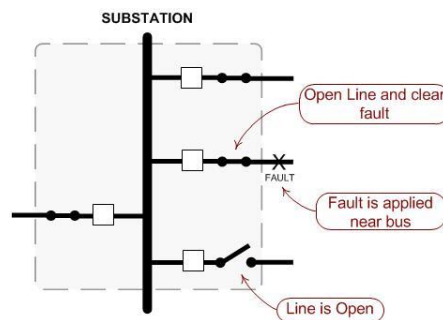
Figure 5.3.3: Event Sequence
