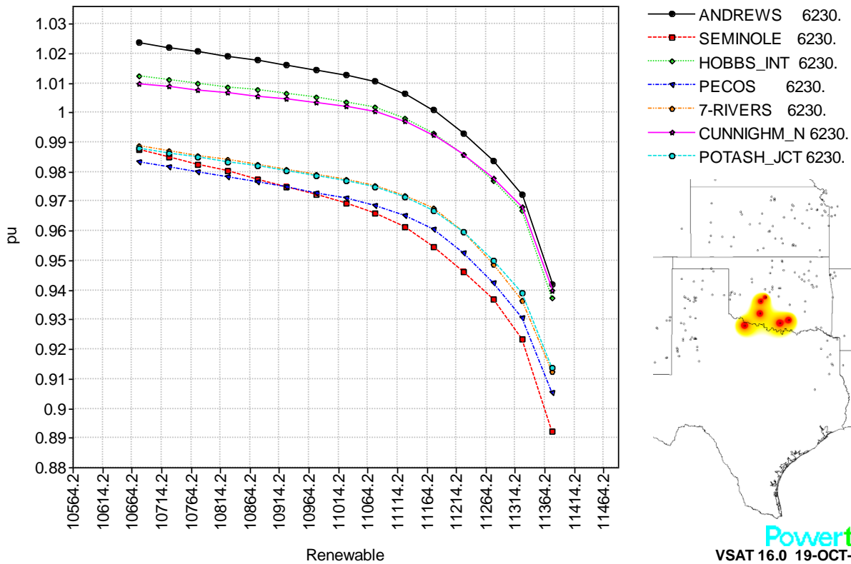
Figure 8.10.2: G-1 P-V Curves
