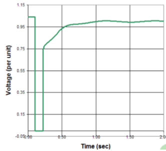
Figure 5.2.3: Transient Voltage Response
