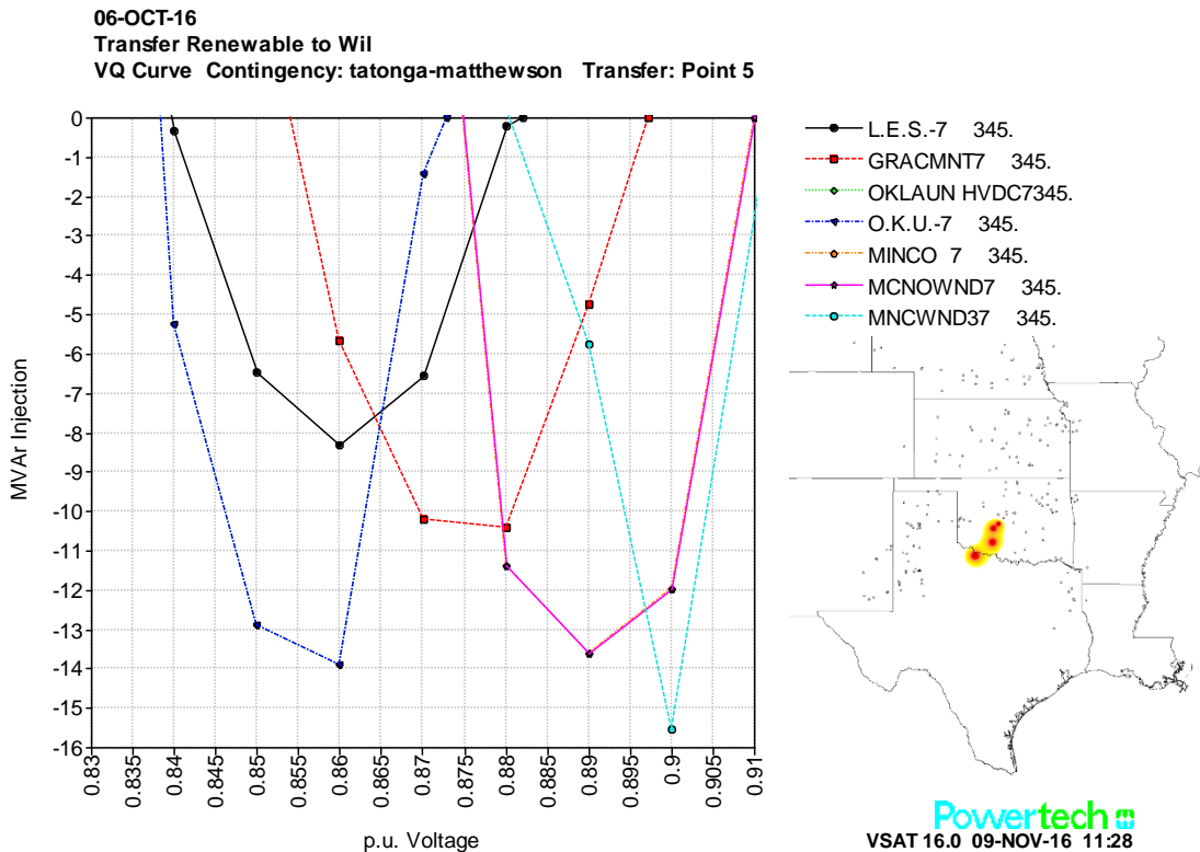
Figure 8.15.7: T-1 Q-V Curves – 95% Point (ATC=161.5MW)
