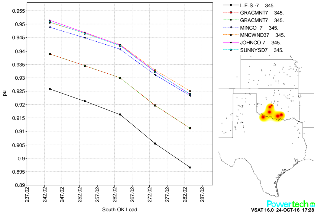
Figure 8.9.2: T-1 P-V Curves
