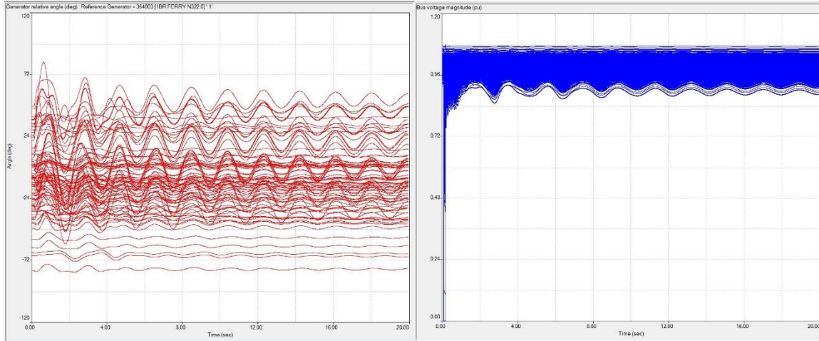
Figure 5.4.12: Machine Rotor Angle – 60% Waverly with Wolf Creek at 900 MW
