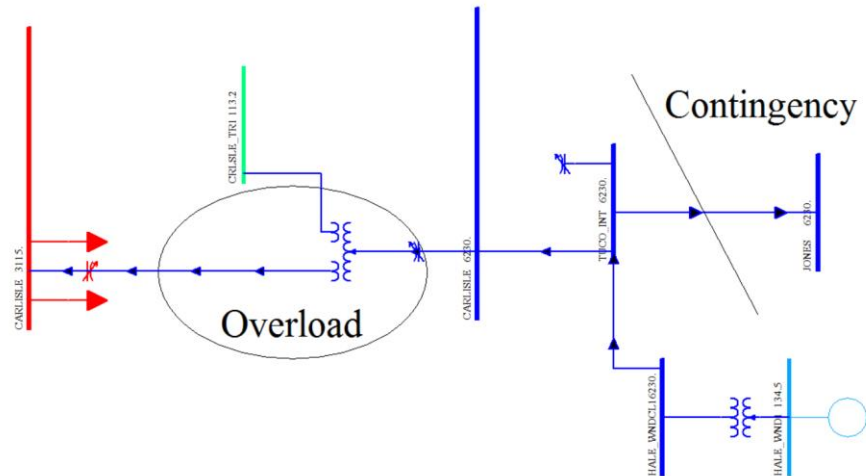
Figure 8.10.13: Worst Overloaded Line and Nearby Wind
