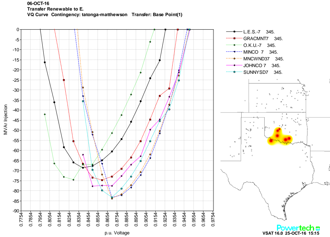
Figure 8.8.6: T-1 Q-V Curves – Base Point
