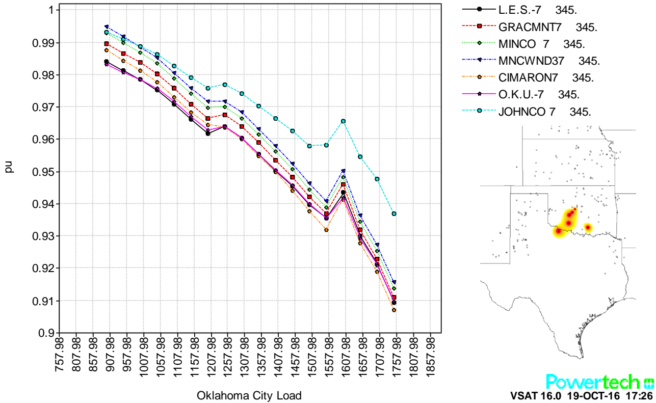
Figure 8.14.1: G-1 P-V Curves
