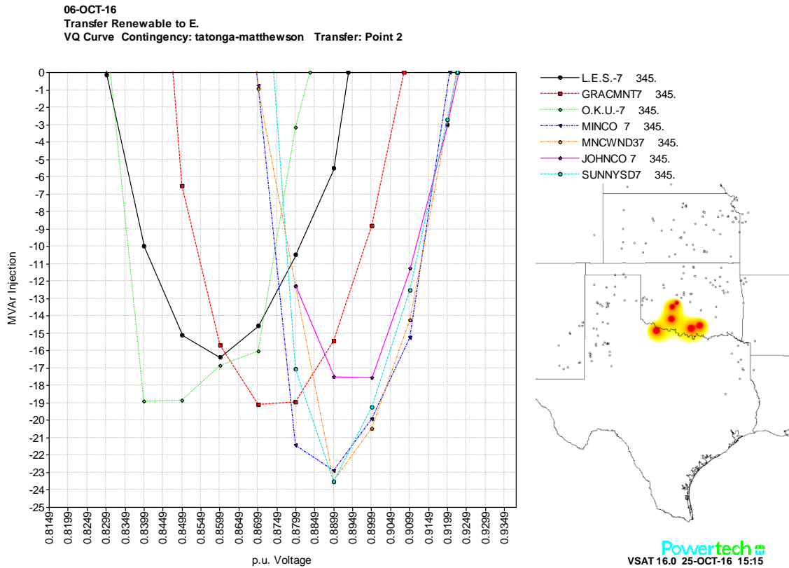
Figure 8.8.7: T-1 Q-V Curves – 95% Point (ATC=161.5MW)
