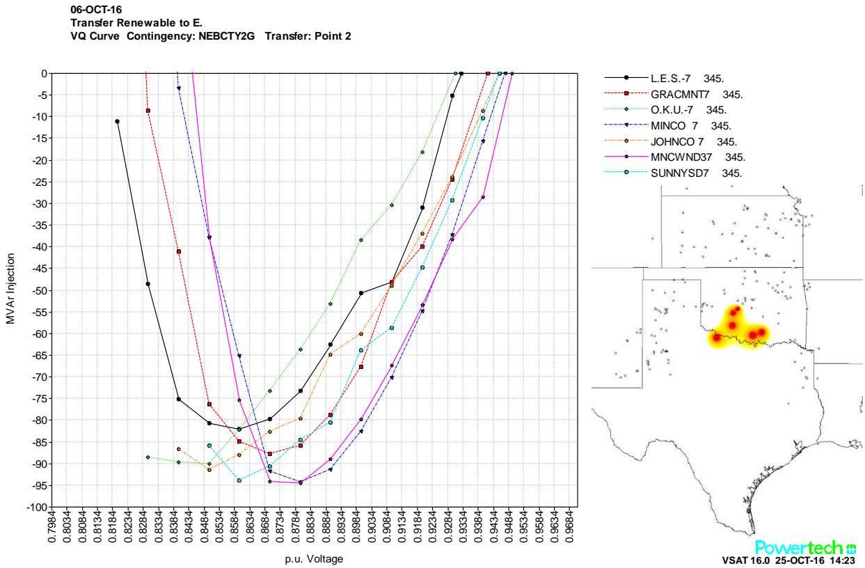
Figure 8.8.5: G-1 Q-V Curves – 95% Point (ATC=1121MW)
