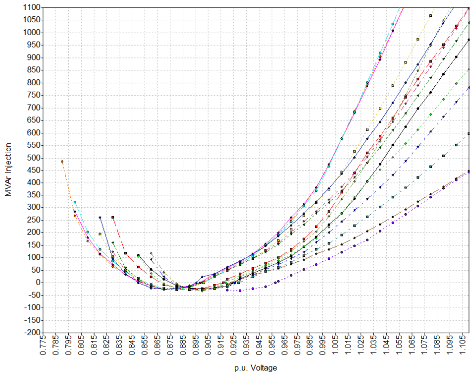
Figure 7.8.4 Q-V curve at the 95% transfer margin
