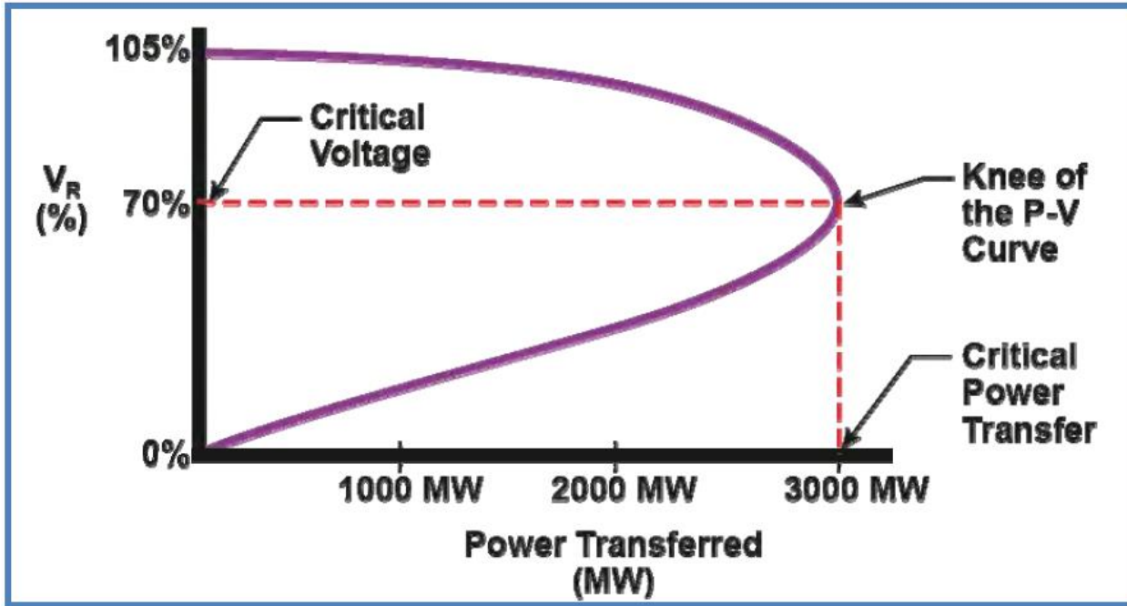
Figure 6.1.1: Sample P-V Curve
