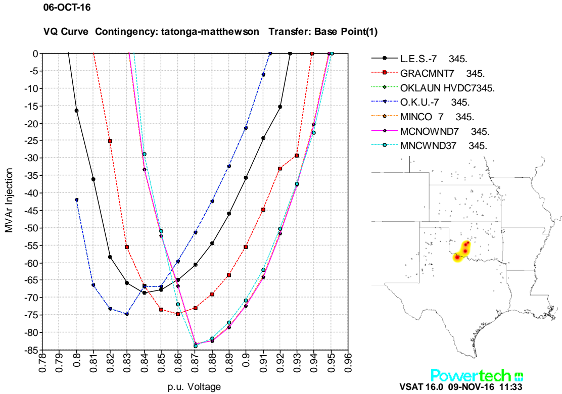
Figure 8.15.6: T-1 Q-V Curves – Base Point
