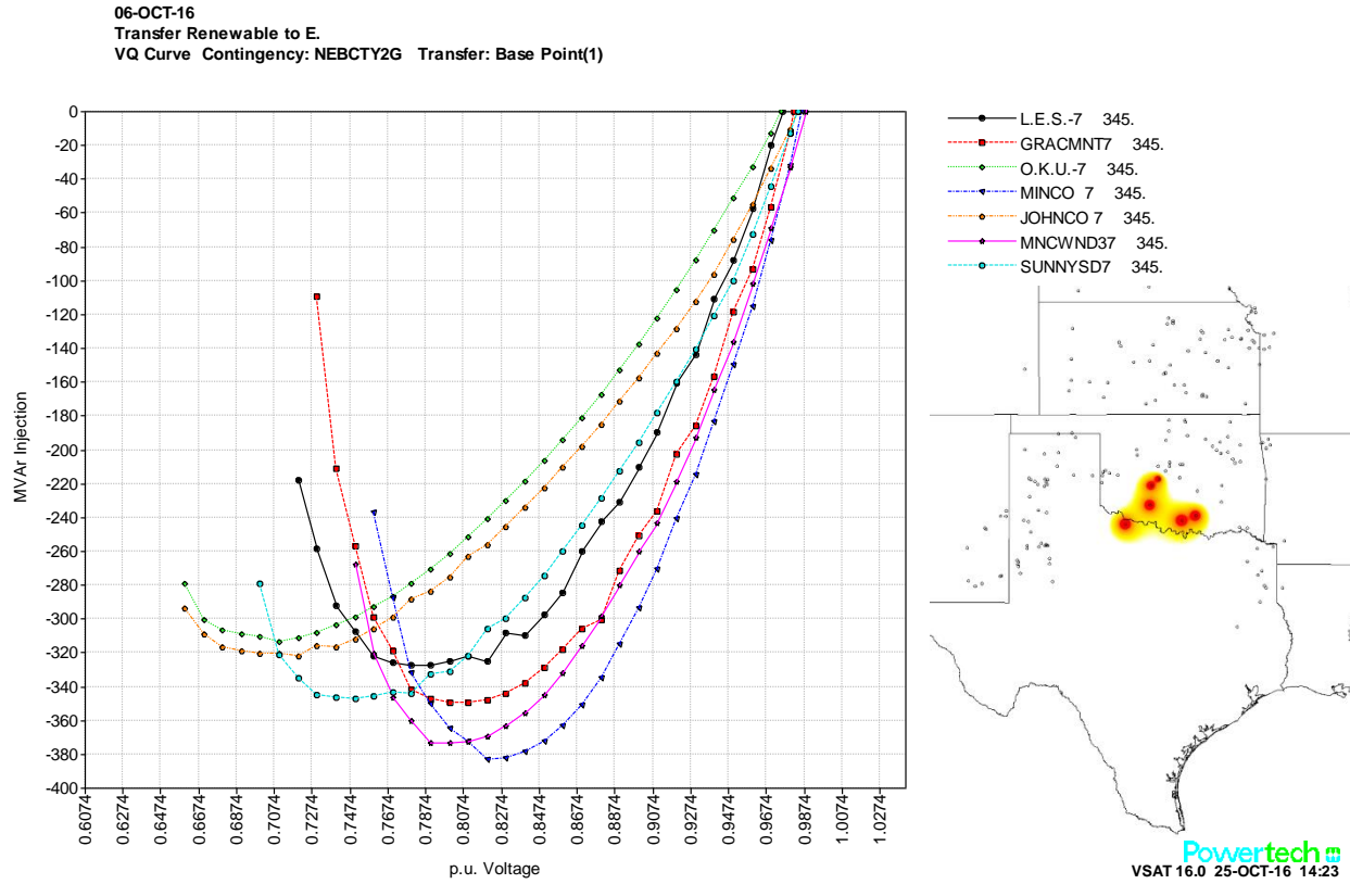
Figure 8.8.4: G-1 Q-V Curves – Base Point
