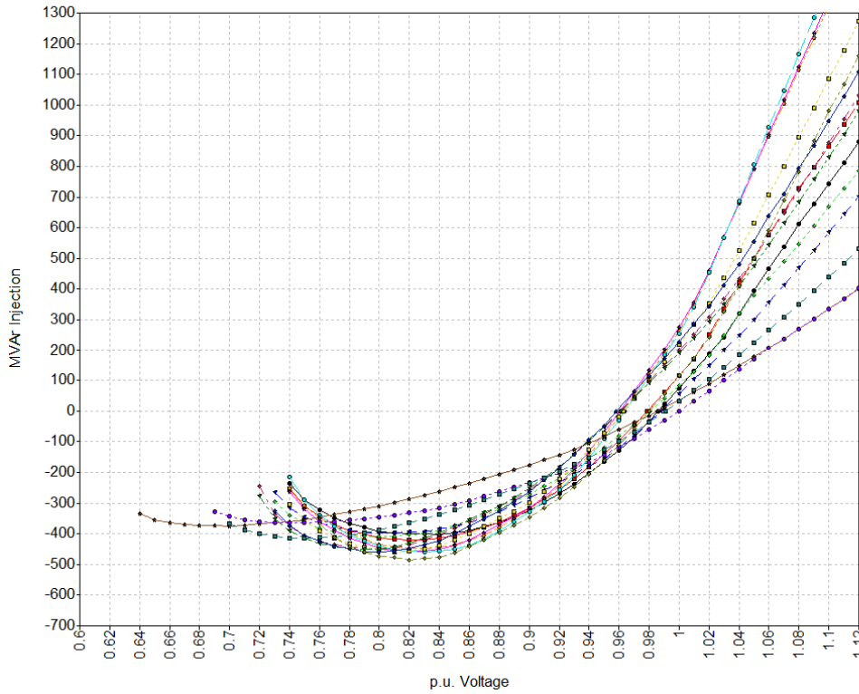
Figure 7.8.3 Q-V curve at the base transfer
