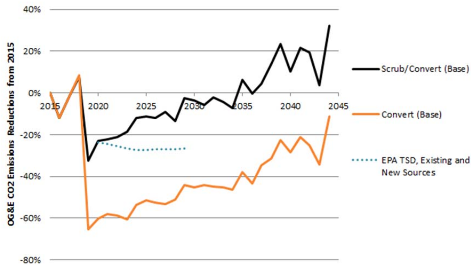
7 Figure 2. OG&E system CO 2 emissions reductions from 2015, EPA rate-to-mass 8 TSD reductions from 2012.
